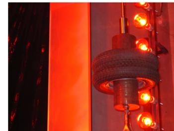
Figure 3.4. Set-up of the impact test represented by Figure 3.3.a (middle point).
