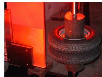
Figure 3.5. Set-up of the impact test represented by Figure 3.3.b (bottom point).
